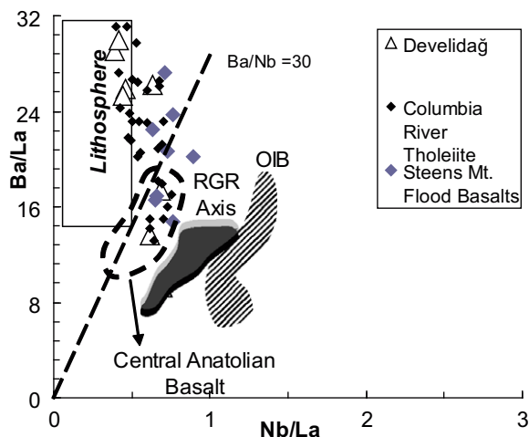
Fig. 8. Ba/La–Nb/La diagram of the Develidağ volcanic rocks. Lithosphere region is from Ormerod et al. (1991). Data sources from Camp et al. (2003), Kürkcüoğlu et al. (2001), Gibson et al. (1993), Chen et al. (1990) Hooper (1988) and Chen and Frey (1985).
